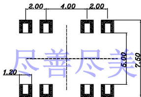
PCB PLERTING PLAN
